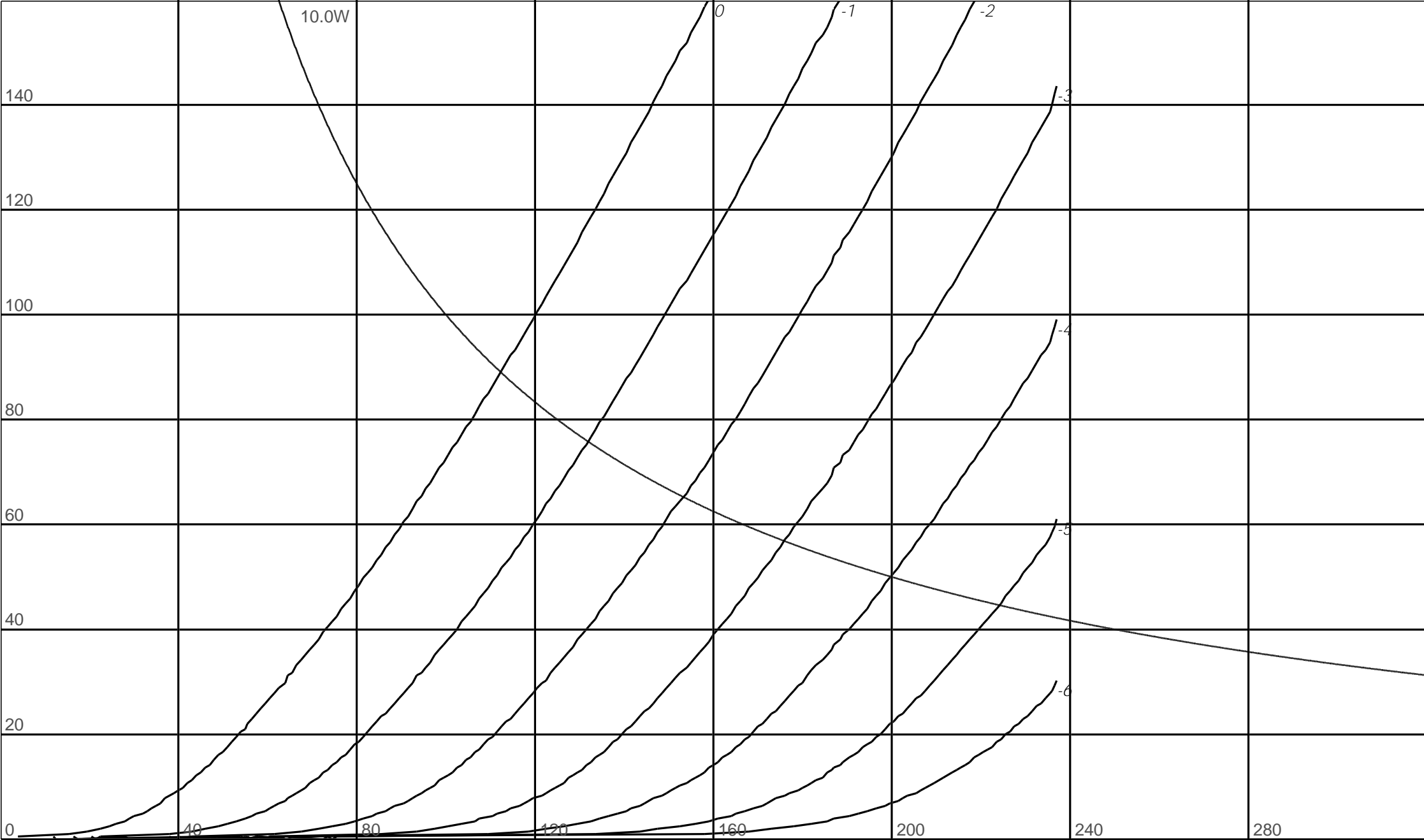
WE418A-1 TRIODE
